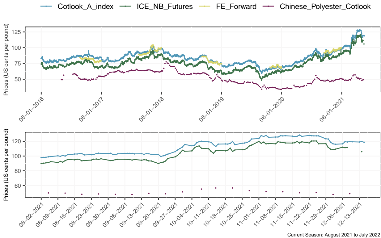
Figure 1: Daily Prices
